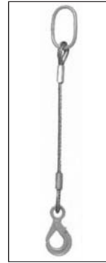
OSL Self-Locking Hook
